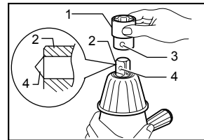
1. Socket 2. Anvil 3. Hole 4. Detent pin
