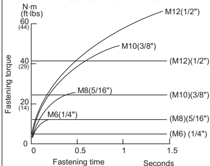
Standard bolt DTD103
