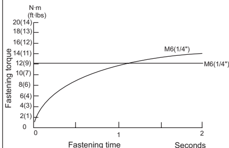
Standard bolt DTD063
