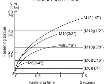
Standard bolt DTD063
